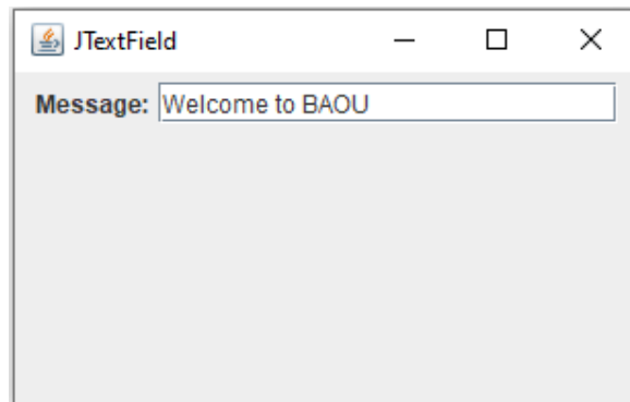
Figure 2. JTextField Example
